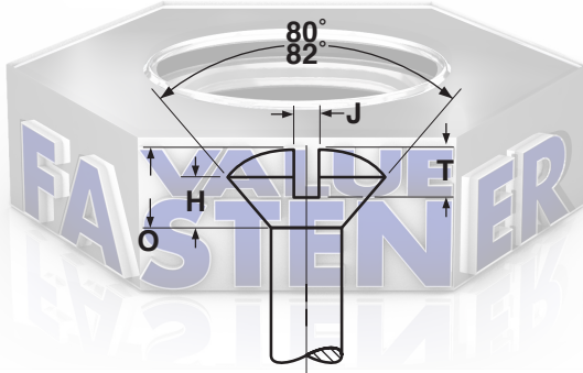
OVAL HEADS FOR WOOD SCREWS
