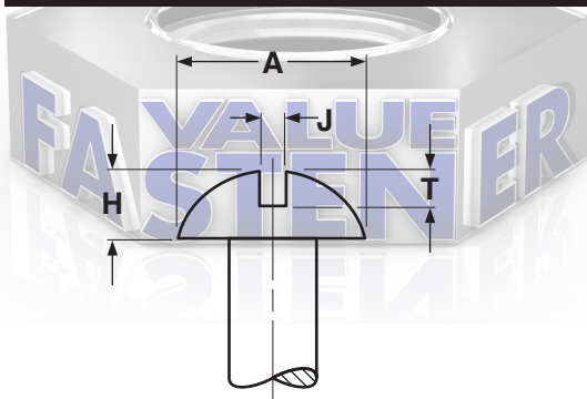
ROUND HEADS FOR WOOD SCREWS
