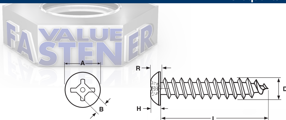
#8 TRUSS w/ #6 HEAD SQUARE-PHILLIPS RECESS DEEP THREAD WOOD SCREW
