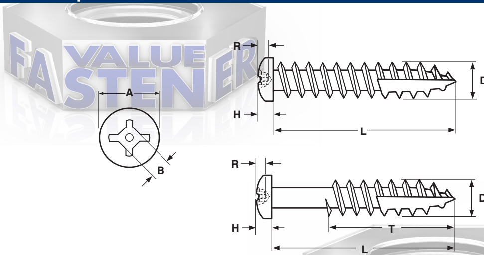
PAN SQUARE-PHILLIPS RECESS DEEP THREAD WOOD SCREW WITH TYPE-17 POINT
