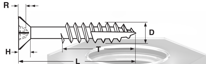
SQUARE-PHILLIPS COMBO FLAT HEAD DEEP THREAD WOOD SCREW—TYPE-17 WITH NIBS
