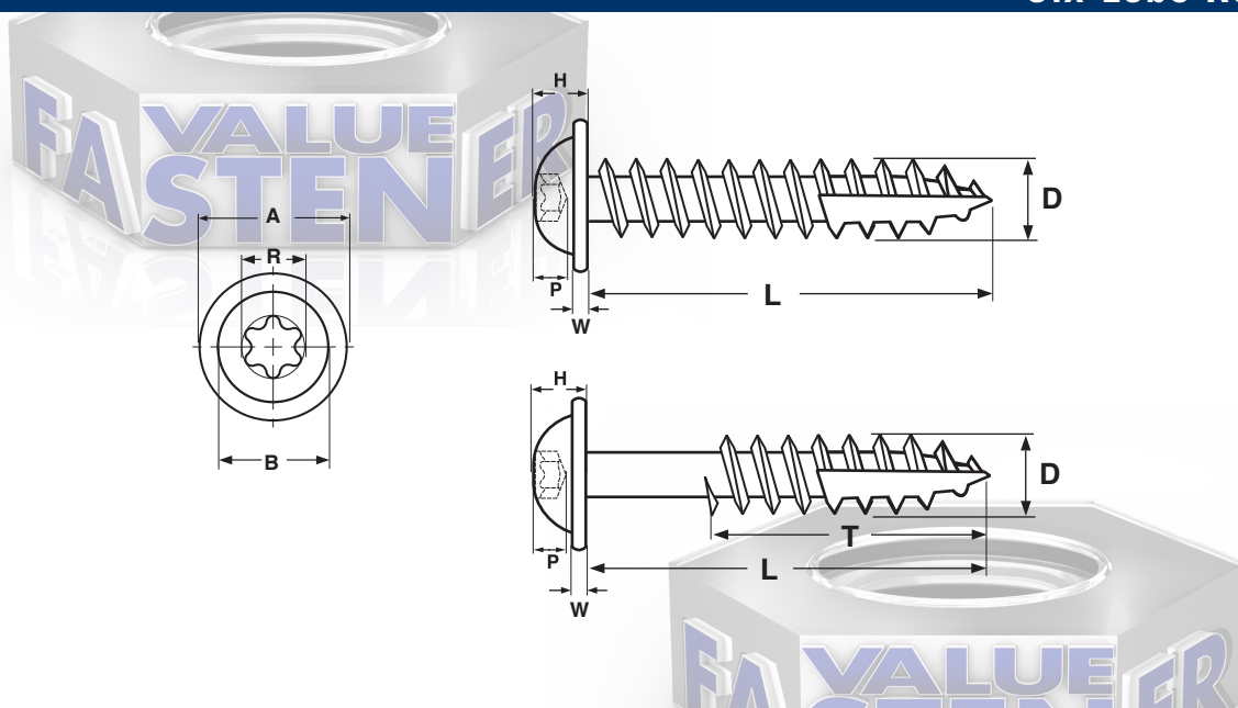
ROUND WASHER SIX-LOBE RECESS DEEP THREAD WOOD SCREW W/ TYPE-17 PT.
