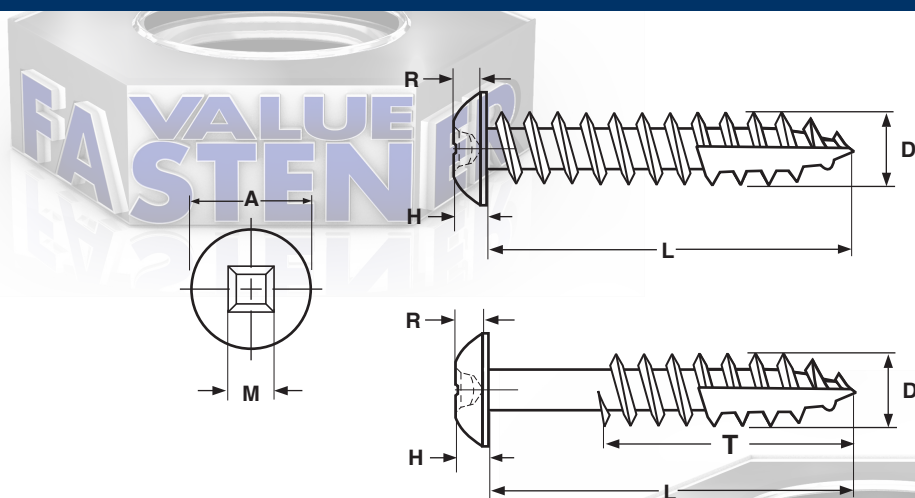
TRUSS SQUARE RECESS DEEP THREAD WOOD SCREW WITH TYPE-17 POINT
