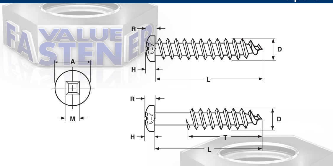
PAN SQUARE RECESS DEEP THREAD WOOD SCREW
