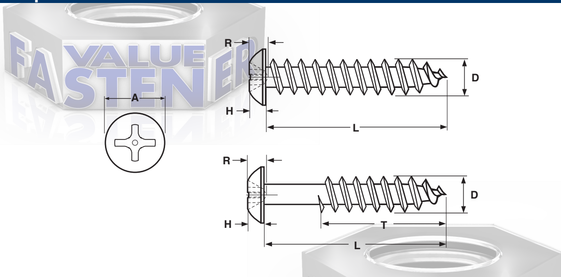
TRUSS PHILLIPS RECESS DEEP THREAD WOOD SCREW
