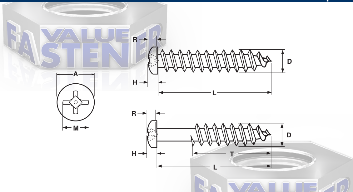
PAN PHILLIPS RECESS DEEP THREAD WOOD SCREW
