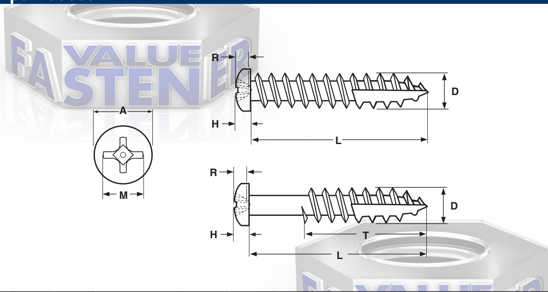
PAN PHILLIPS RECESS DEEP THREAD WOOD SCREW WITH TYPE-17 POINT
