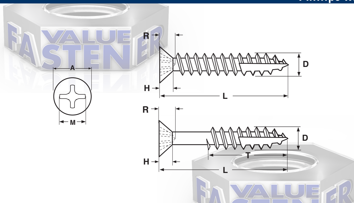
FLAT PHILLIPS RECESS DEEP THREAD WOOD SCREW WITH TYPE-17 POINT
