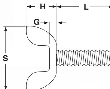
WING SCREWS - STAMPED STYLE
