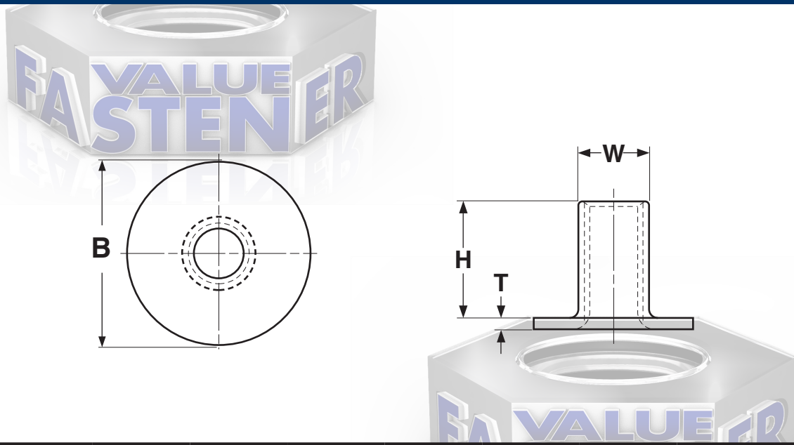
ROUND BASE WELD NUTS WITHOUT PROJECTIONS
