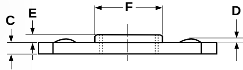
TAB WELD NUTS - CENTER HOLE DESIGN WITH MULTIPLE PROJECTIONS
