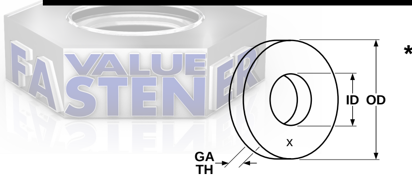
USS THROUGH-HARDENED FLAT WASHERS
