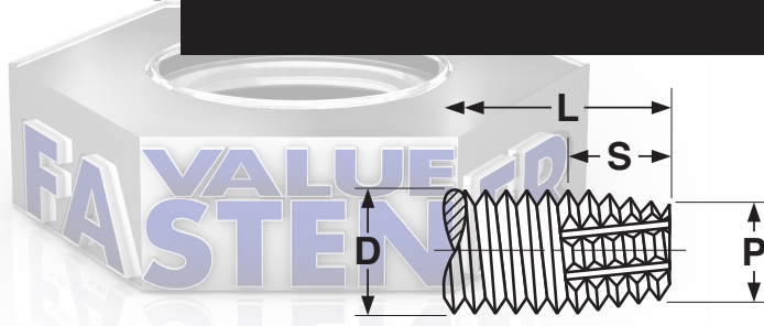
THREADS AND POINTS FOR TYPE-F THREAD CUTTING SCREWS
