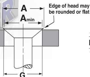
FLAT HEAD 100° FOR SELF-TAPPING SCREWS
