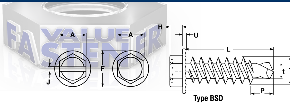
SERRATED HEX WASHER SELF-DRILLING SCREWS, SPACED THREAD
