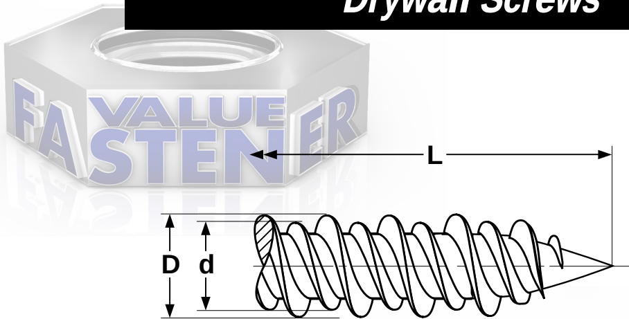
High-Low Pattern Drywall Screw Thread
