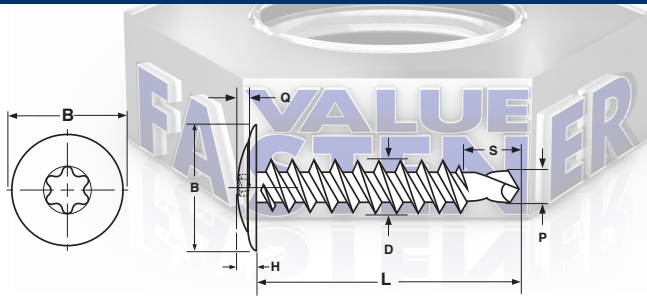
Six-Lobe Recess
