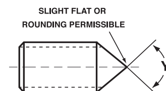
CONE POINT
