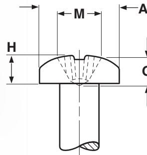
METRIC - TYPE Z (1A) PAN HEADS FOR TAPPING SCREWS
