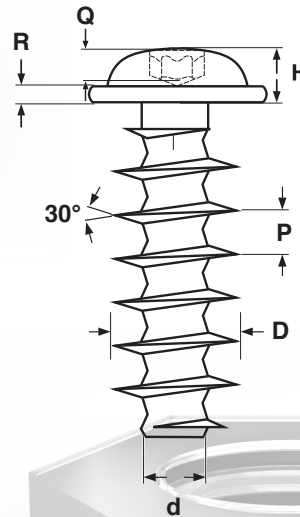
METRIC - TYPE PT®-ALTERNATIVE THREAD FORMING SCREWS, ROUND WASHER 6-LOBE
