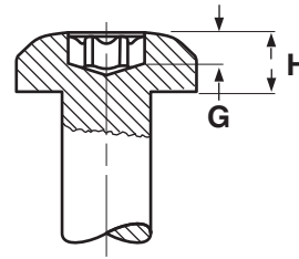
METRIC - ISO 14583 PAN SIX-LOBE MACHINE SCREWS
