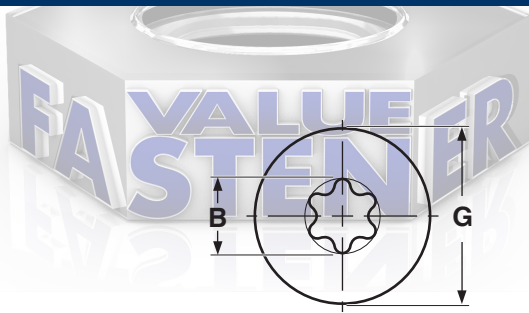
METRIC - ISO 14581 90° FLAT SIX-LOBE MACHINE SCREWS
