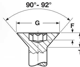
METRIC - ISO 14581 90° FLAT SIX-LOBE MACHINE SCREWS
