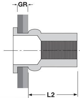
FLAT HEAD, NON-RIBBED BLIND THREADED INSERT
