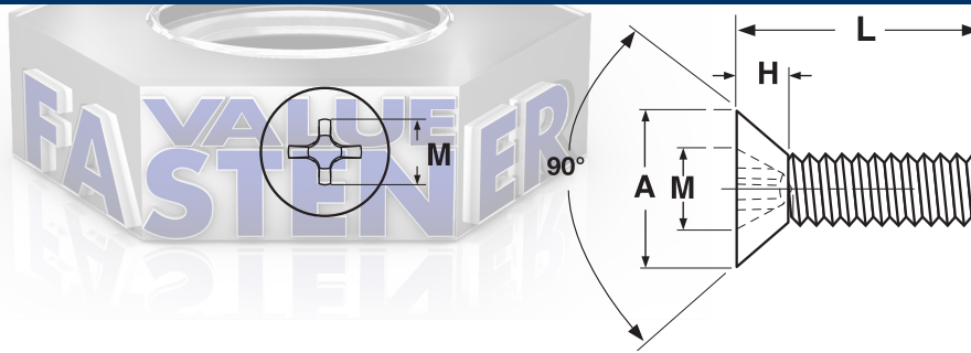
DIN 965 90° FLAT PHILLIPS (TYPE H RECESS) MACHINE SCREWS
