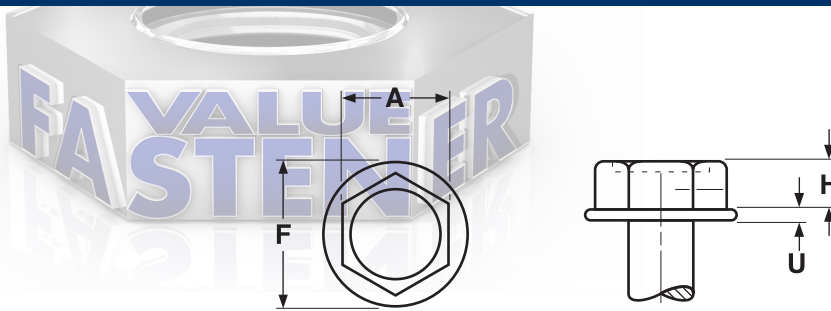
METRIC - UNSLOTTED HEX WASHER DIN 7500~D HEAD
