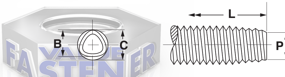
METRIC - TRILOBULAR THREAD ROLLING SCREWS
