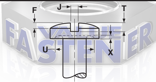
SLOTTED BINDING HEADS UNDERCUT FOR MACHINE SCREWS
