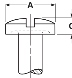
SLOTTED BINDING HEADS UNDERCUT FOR MACHINE SCREWS
