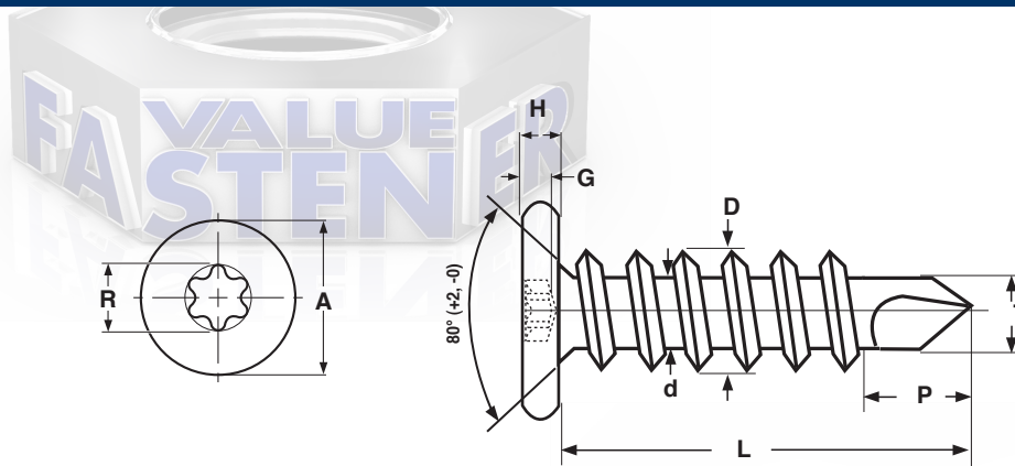
PANCAKE SIX-LOBE SELF-DRILLING SCREWS, SPACED THREAD AND #3 DRILL POINT
